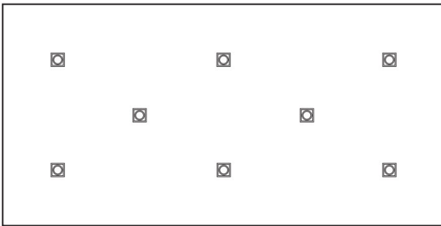
8 per 4x8 board with Adhered Reinforced Membrane (TPO, PVC, EPDM-R, Mod Bit)
